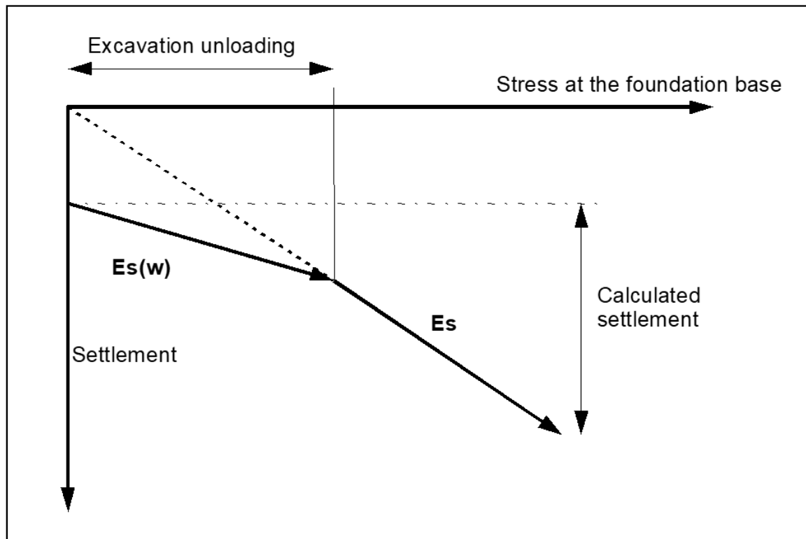
Figure 4 Excavation unloading and constrained modulus
